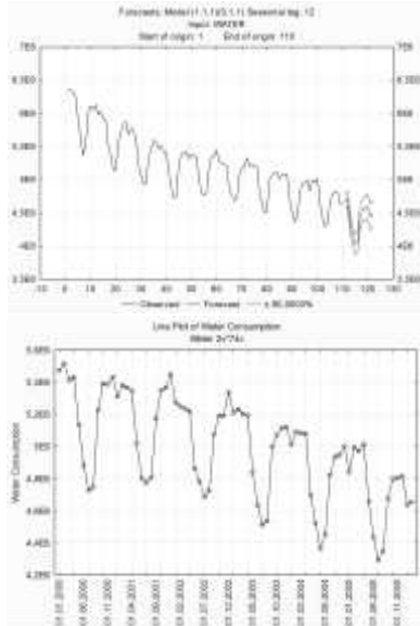
Figure 9. Comparison of "retro forecast" and real data charts
