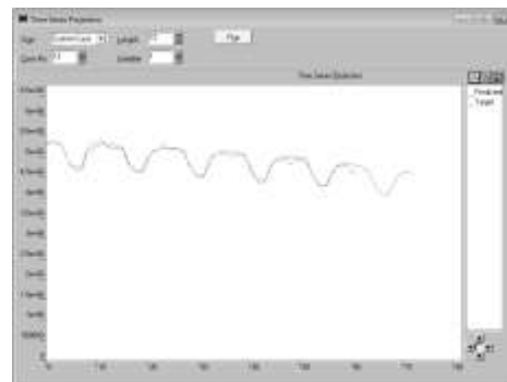
Figure 13. The projection of time series forecast results for 12 months
