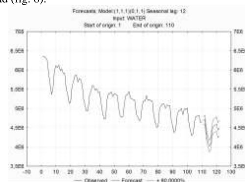
Figure 6. Chart of forecasting for 12 months using ARIMA model (1,1,1) (0,1,1)
