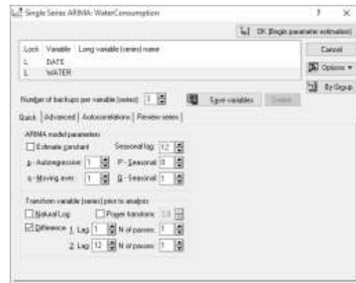
Figure 5. Setting up ARIMA model (1,1,1) (0,1,1)
