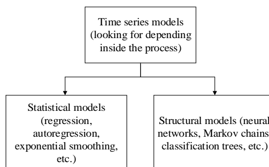
Figure 1. Classification of time series models
