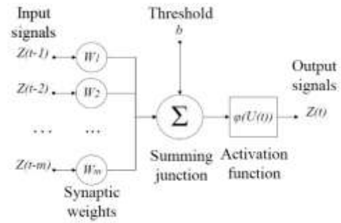
Figure 2. Nonlinear neuron model
