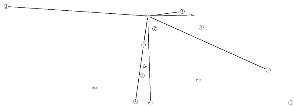
Fig. 6. General view of the non-orientated link graph for backlink insurance companies
