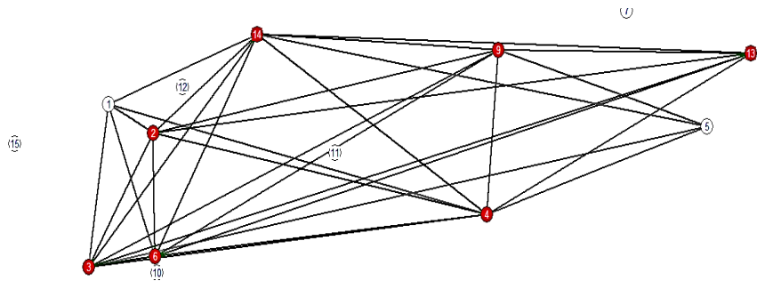
Fig. 5. Finding the maximum click on the insurance company relationship graph
