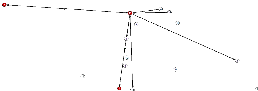
Fig. 7. Highlighting the path of achievement from top №2 to top №5, which are insurance companies (2) and (5)
