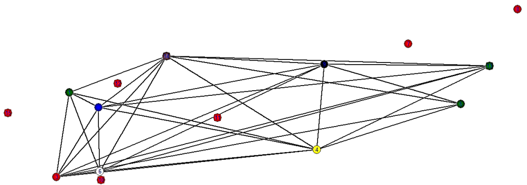
Fig. 4. Selection of contours or cycles that can be created by insurance companies
