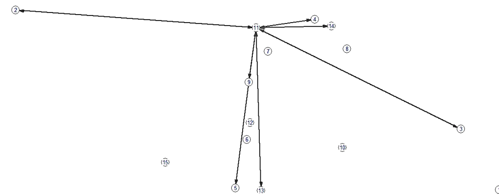
Fig. 8. Type of an oriented graph of relationships of insurance companies
