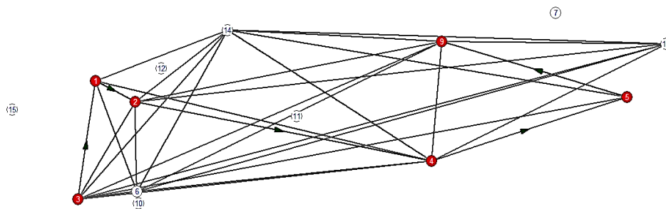
Fig. 2. Highlighting the path of achievement from top № 3 to top № 9
