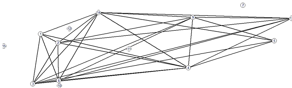
Fig. 1. General view of a non-orientated link graph for direct-link insurance companies
