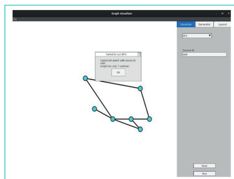
Figure 5. BFS algorithm input validation
