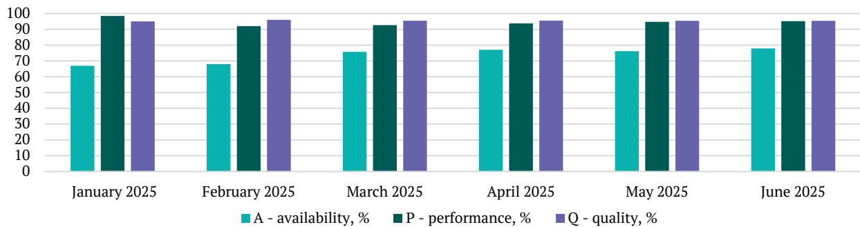
Figure 2. Components of overall equipment effectiveness for “Tube Plant” LLC
