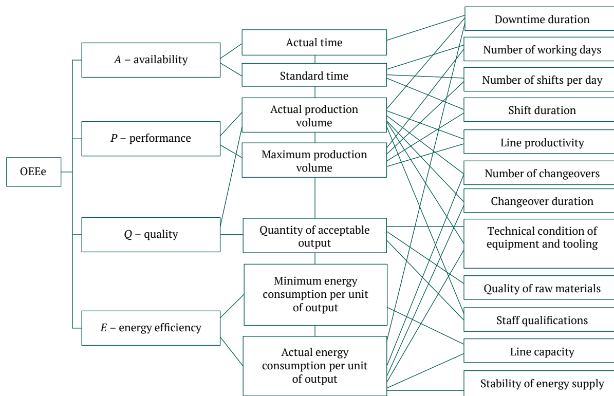
Figure 4. Factors affecting the level of OEEe
