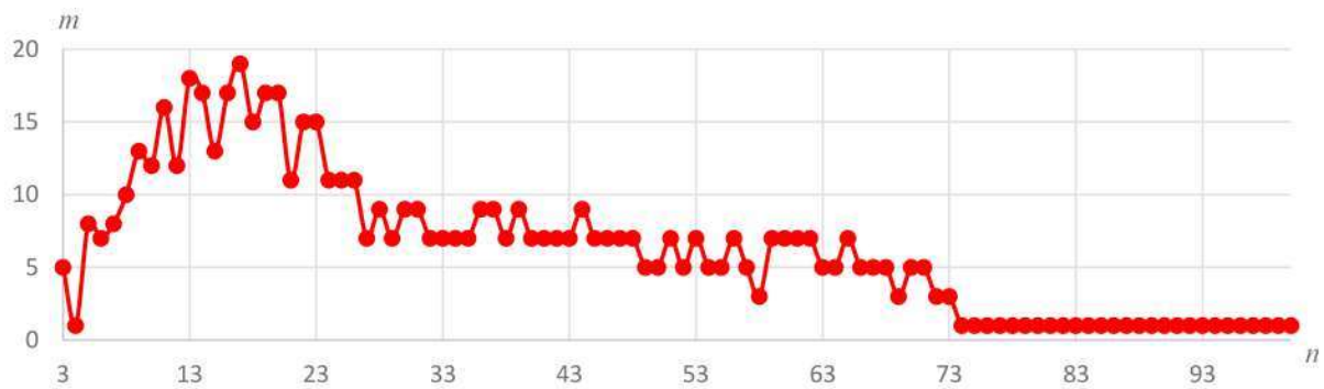
Fig. 17. The number of partition trajectories in the circle-based partitioning algorithm for the curve shown in Fig. 16, as the number of segments varies from 3 to 100, with allowable chord length deviation \varepsilon = 0.0001 and n_1 = \lfloor n/2 \rfloor
