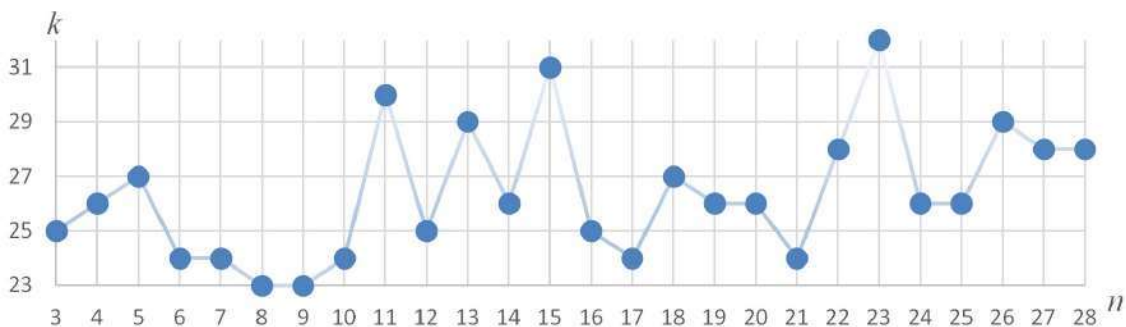
Fig. 14. The number of iterations of the circle-based partitioning algorithm for the curve in Fig. 5 as the number of segments varies from 3 to 28, with allowable chord length deviation \varepsilon = 0.0001 and n_1 = \lfloor n/2 \rfloor
